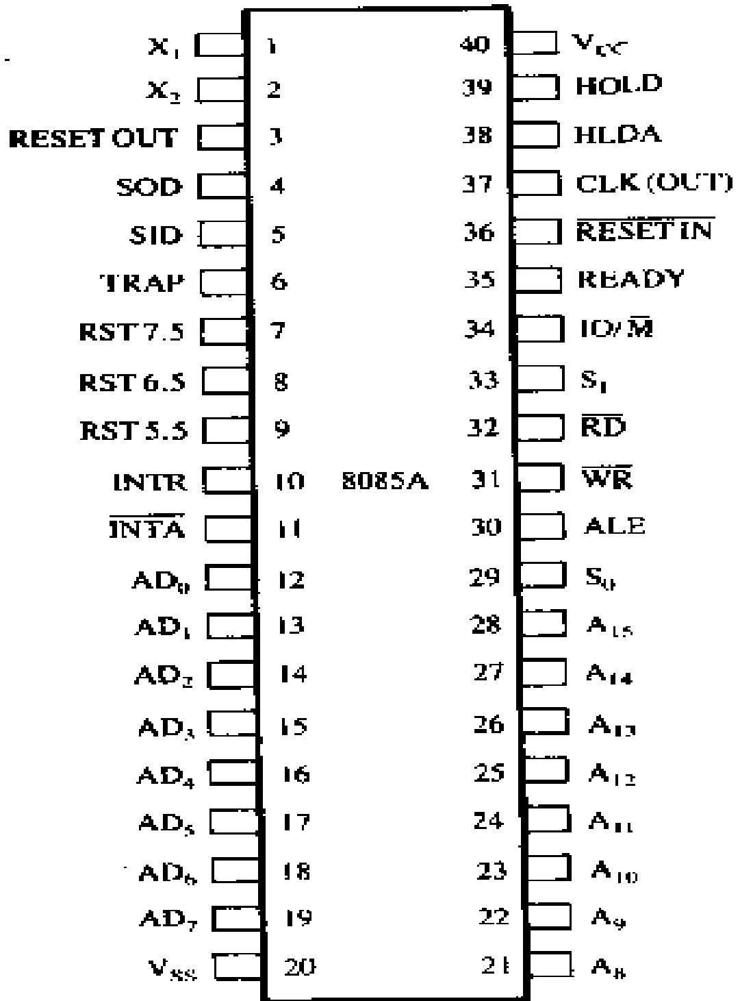
8085 Pinout
